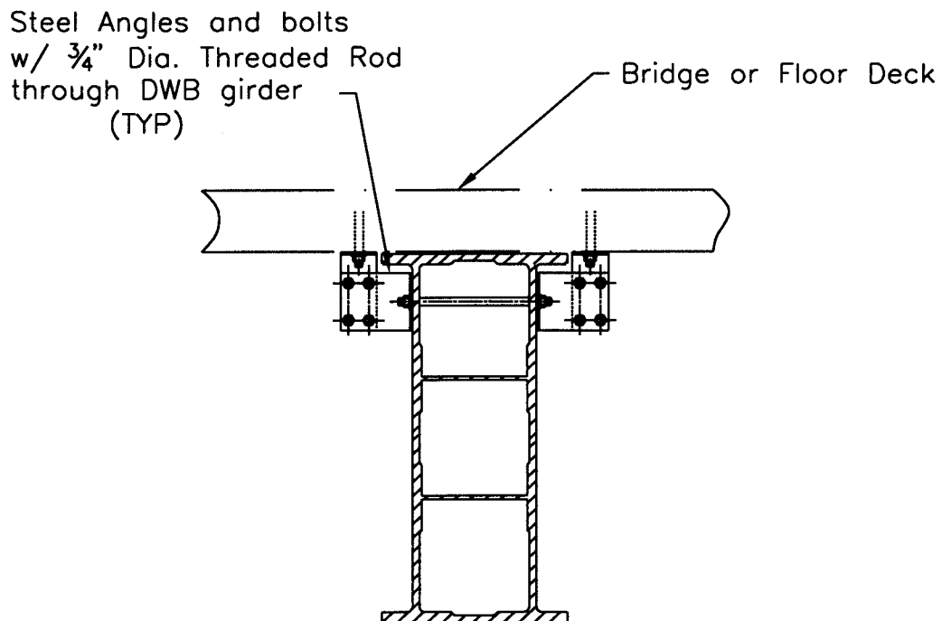
Figure 28. Deck Connection
